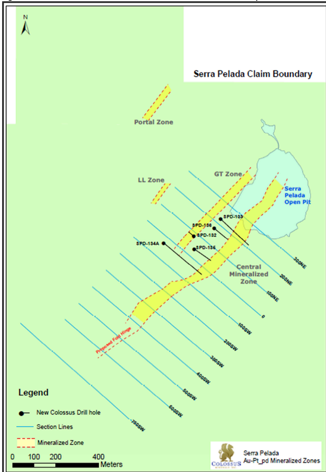
Figure 3: Plan View of Serra Pelada Mineralized Zones with location of reported holes.
