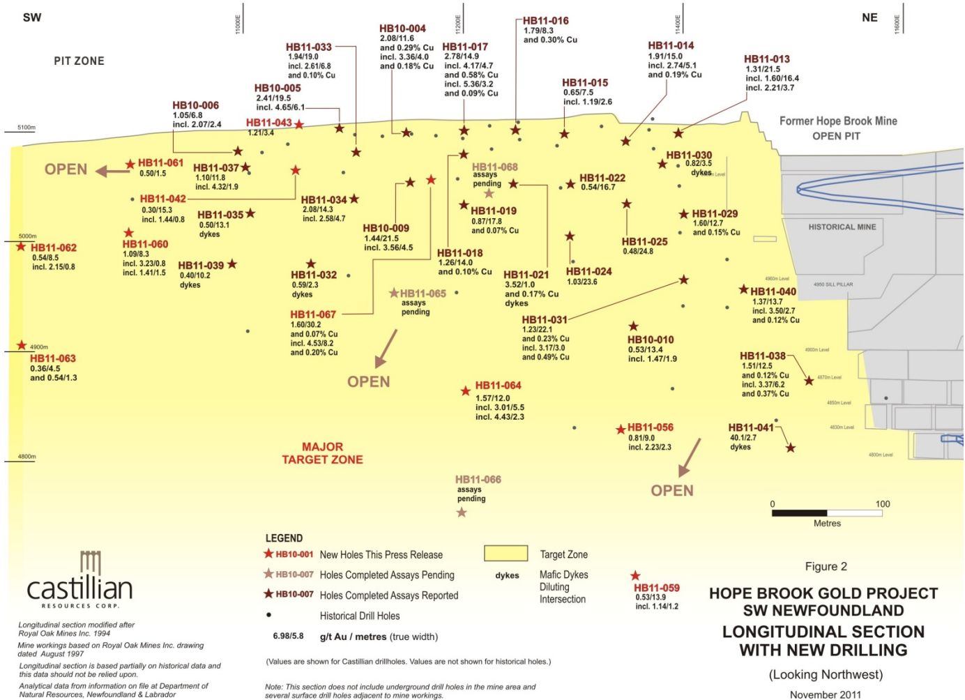
Figure 2. Vertical Longitudinal Section, Pit Zone – Mine Zone Extension
