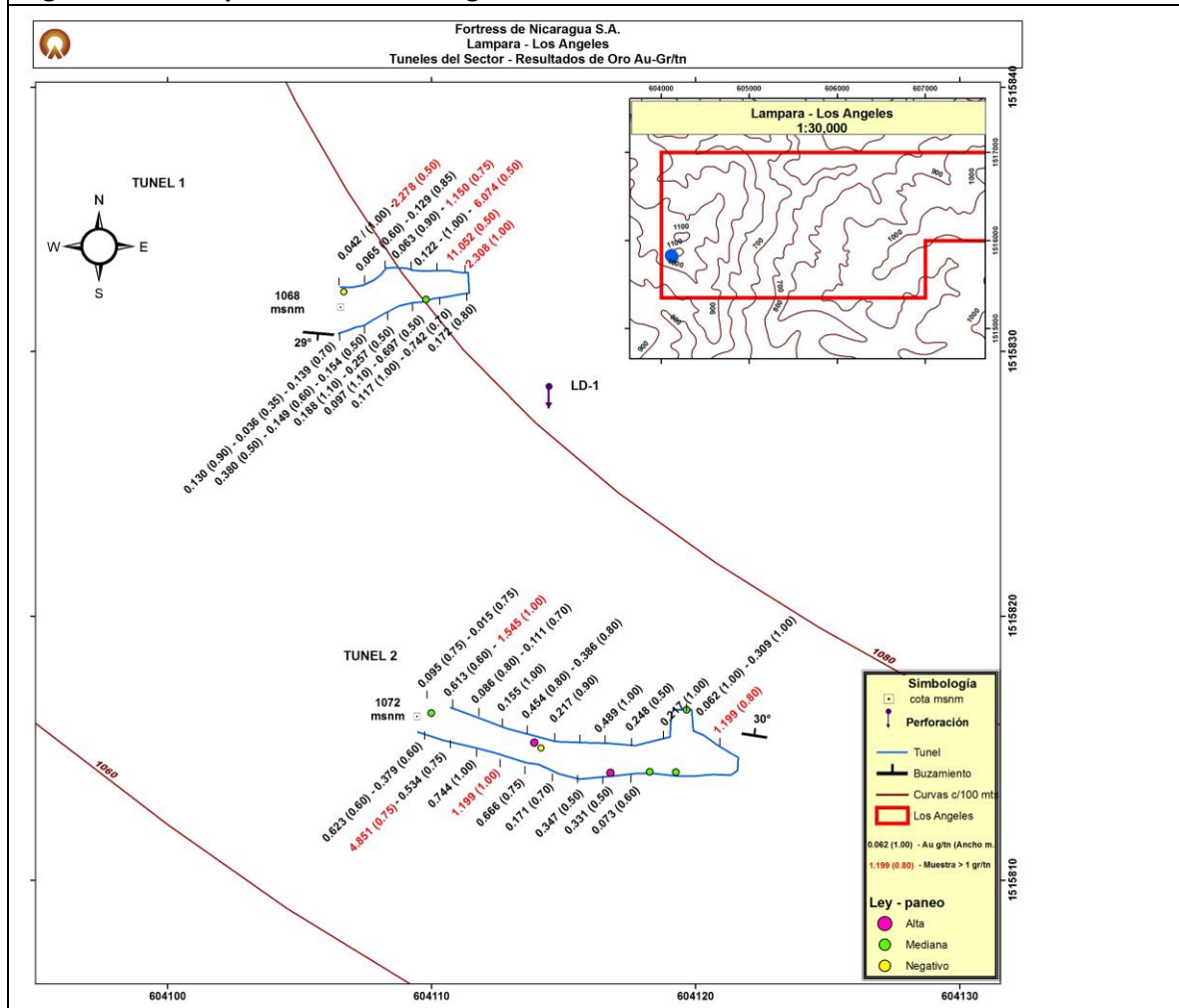
Figure 1 : La Lampara Tunnel Workings
