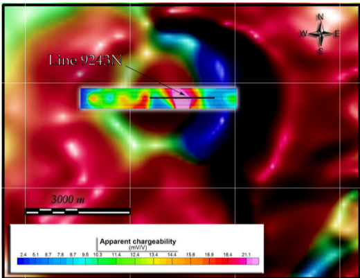
Figure 1: Camargo project, Chargeability anomaly over regional airborne magnetics
