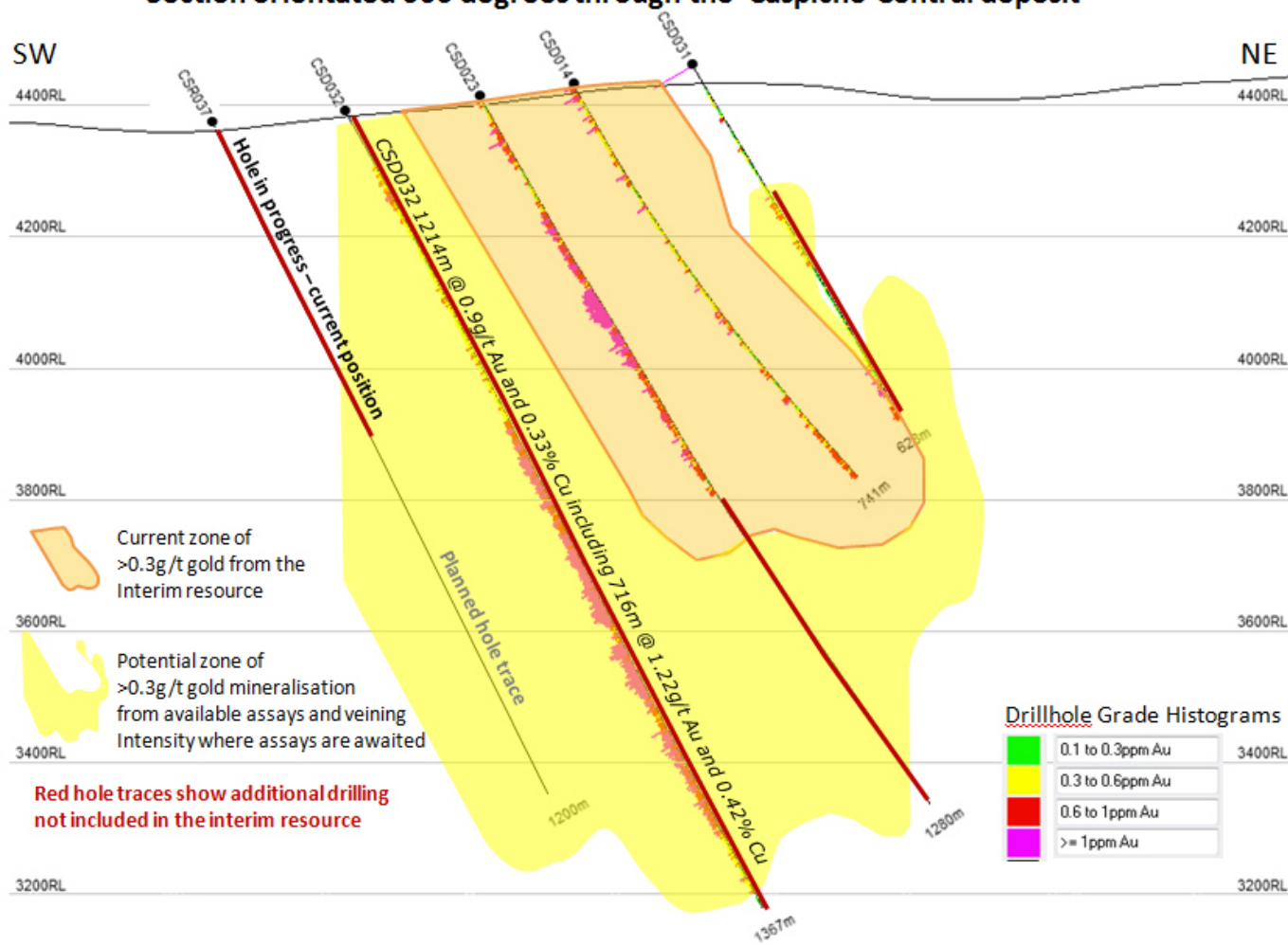
Drill Section Above: shows results and interpreted gold mineralization contours for holes, CSR037, CSD032, CSD023, CSD014 and CSD031.
