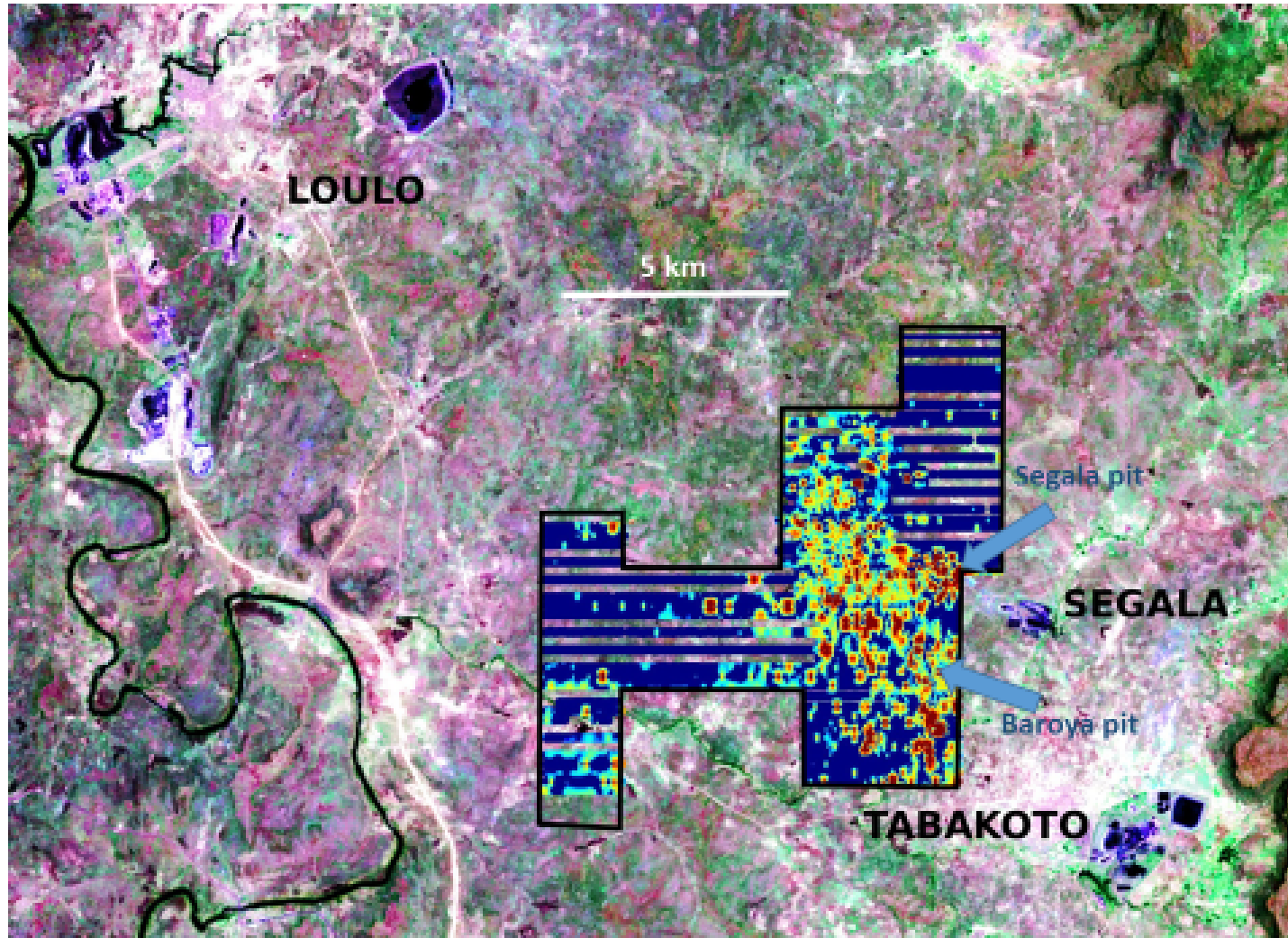
Figure 1. Satellite image of the Segala Ouest project area. Infill colours are relative soil geochemical values with the blue colouration being background below 20 ppb Au. The yellow to red colours reflect the spread of anomalous values. The neighbouring producing mines are identified, viz.: Endeavour's Segala and Tabakoto mines (with a published resource of 3.28 Moz) and Randgold's Loulo-Goukoto mine complex (with a published resource of 13.4 Moz).
