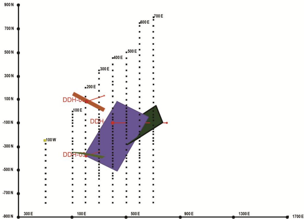
Plan view of the modelled conductors as well as tracing of the drillings
