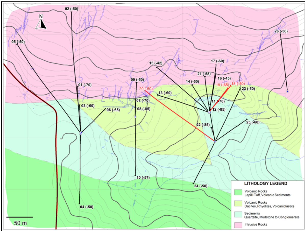
Figure 1: Location of drill holes and interpreted geology map.
