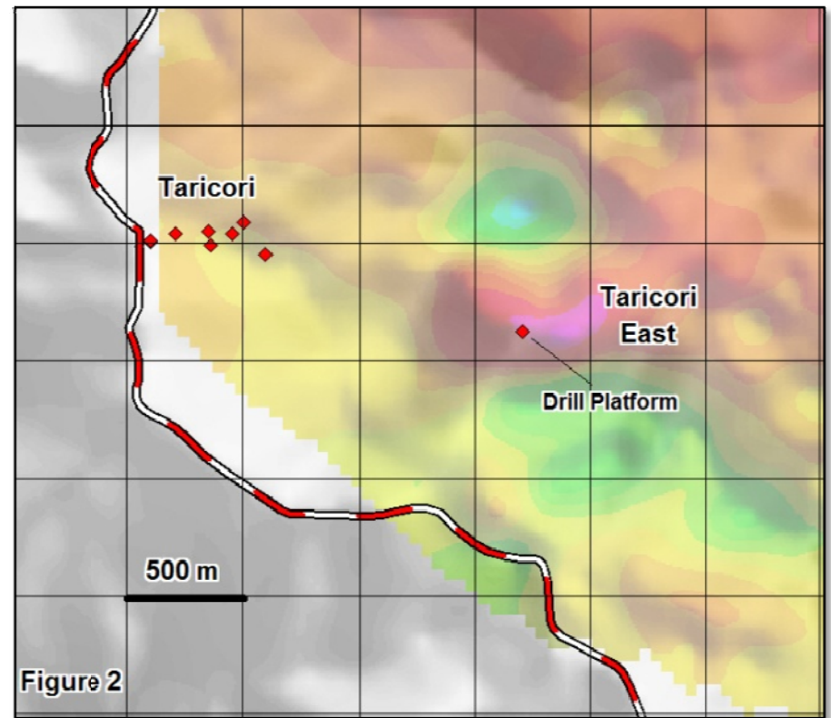
Figures 1 & 2: Location of the Taricori East Drill Target (Canelo geophysical anomalies). Figure 1 shows electromagnetic response (EM-Z4) and Figure 2 shows magnetic response.
