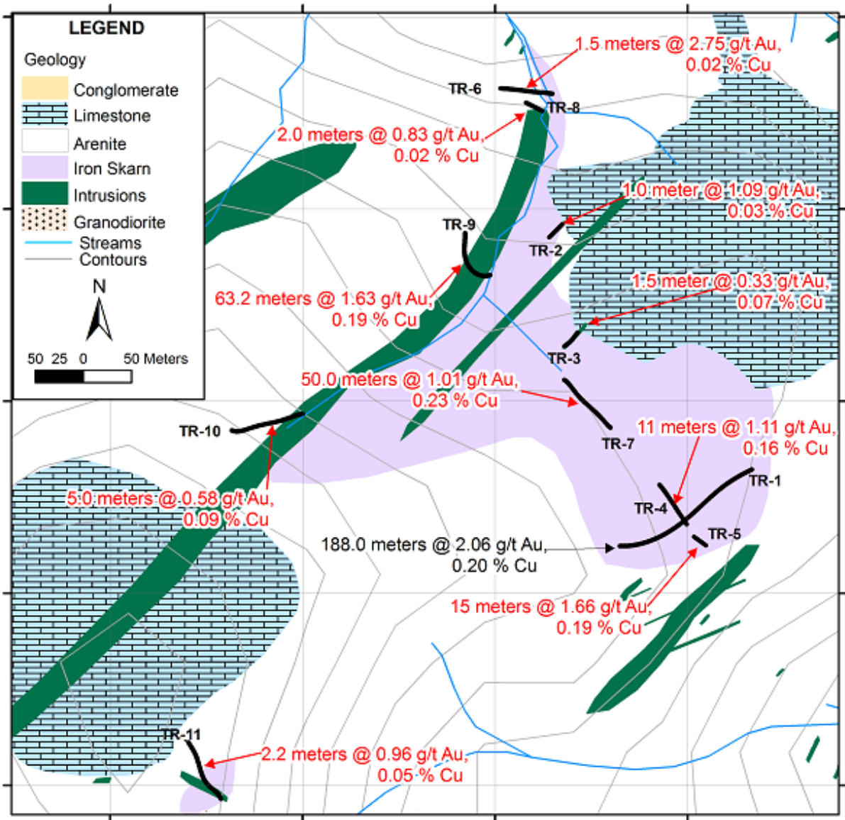
Figure2. Gold and copper intercepts and trench distribution for Trenches 1 through 11.
