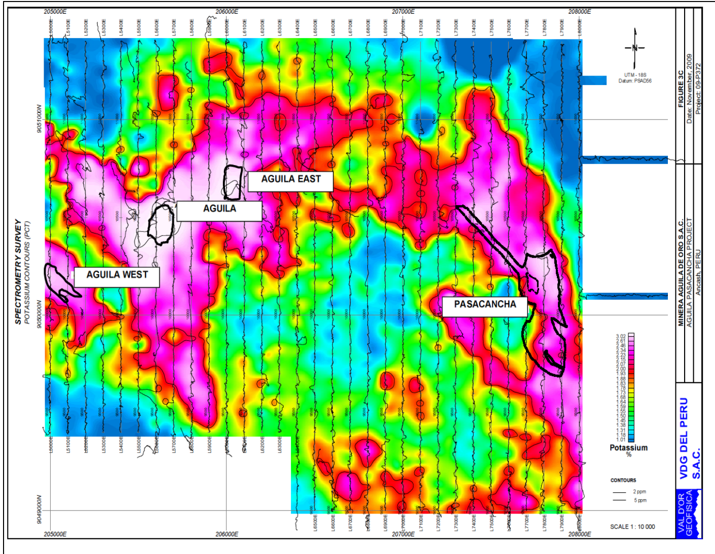
MAP 1. Spectrometry with Potassium (K) – Widespread alteration zone highlighted by red-pink-white colors. Note large area compared to known zones of mineralization.
