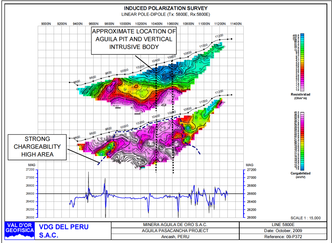
SECTION 4. Resistivity (top) and IP Chargeability (bottom) Pseudosection at Line 5800 E, to East of Aguila Pit: Intense chargeability high extending 600 metres to south and 200 metres to north of Aguila intrusive
