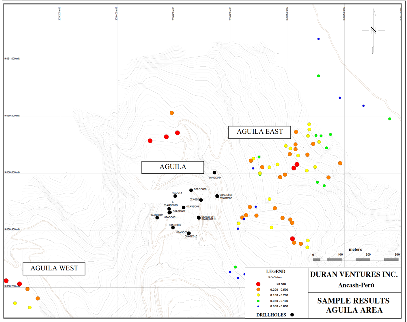
MAP 5. Copper results from first 74 surface samples collected in the Aguilá area.
