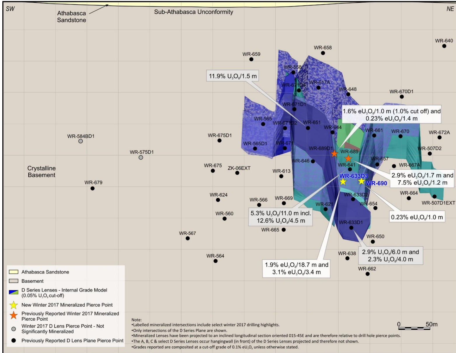
Figure 5: Inclined longitudinal section of the Gryphon D series lenses.
