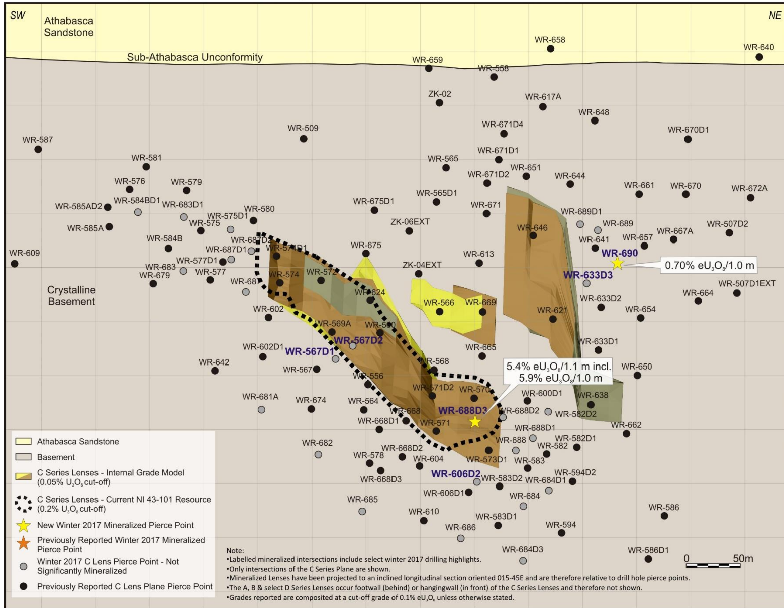
Figure 4: Inclined longitudinal section of the Gryphon C series lenses.
