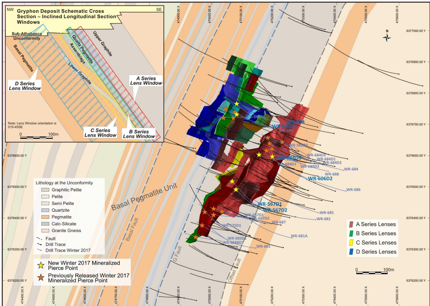
Figure 1: Plan map of the northeast plunging Gryphon mineralized lenses projected up to the simplified basement geology at the sub-Athabasca unconformity.
