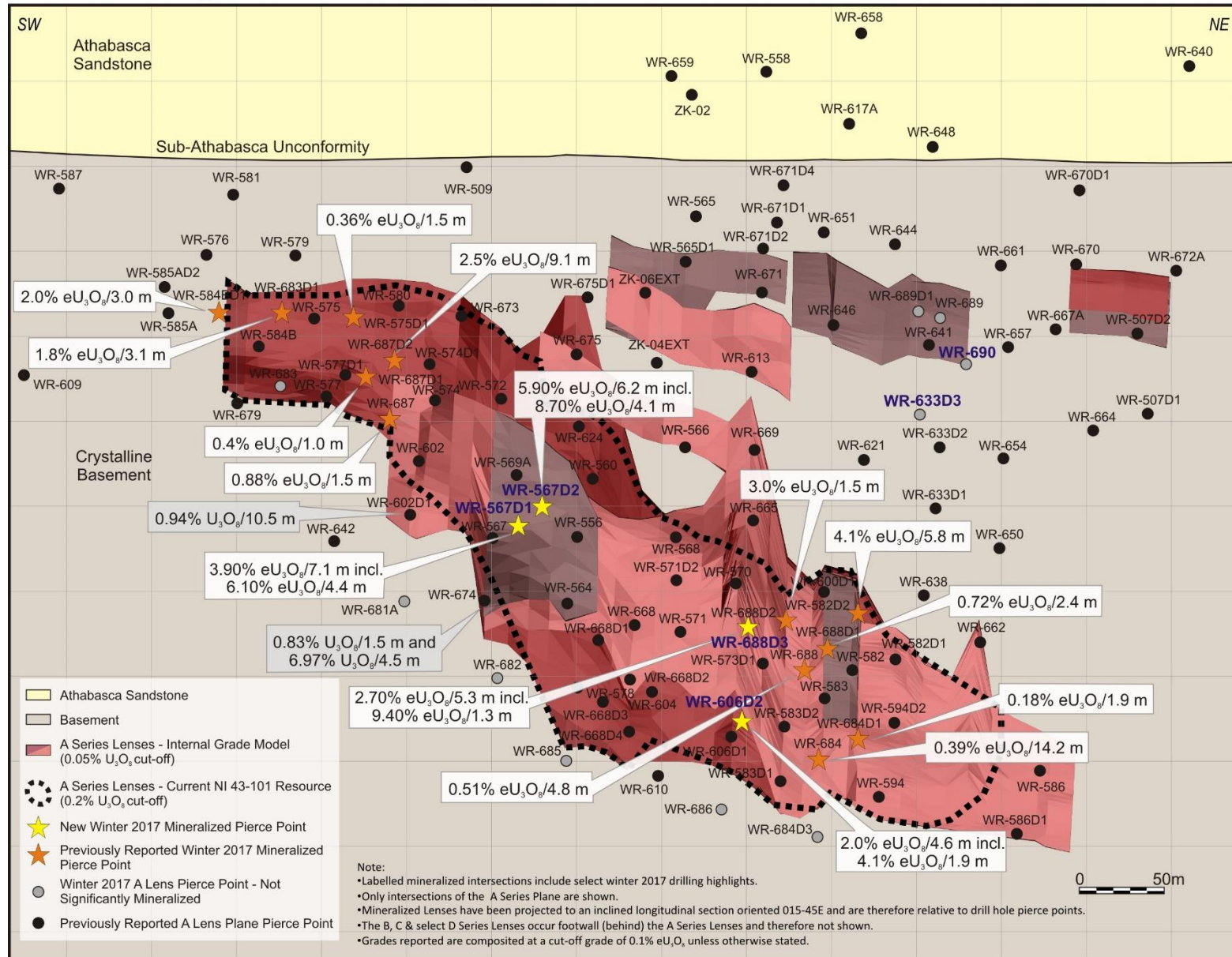
Figure 2: Inclined longitudinal section of the Gryphon A series lenses.
