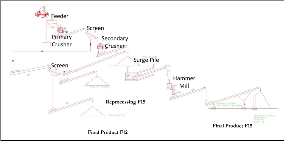
Figure 1 Natural Phosphate Processing Flowchart
