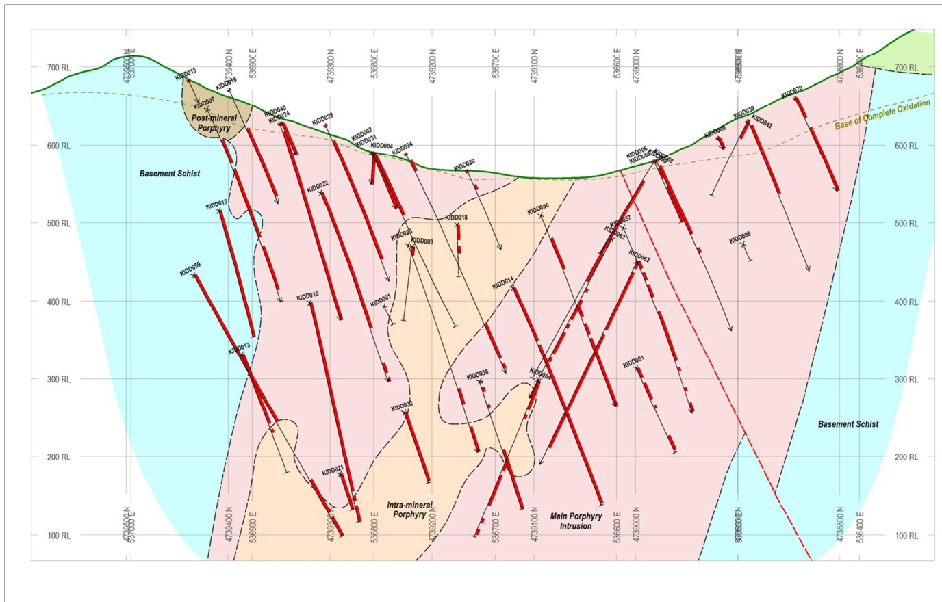
Figure 3: Shows a representative northeast-southwest cross-section (looking southeast) through the Kiseljak area with all drill hole intersections (0.26% CuEq cut-off) and summary geology based on Dunav’s understanding to date. Note that copper-gold mineralization remains open at depth across a significant majority of the cross-section.
