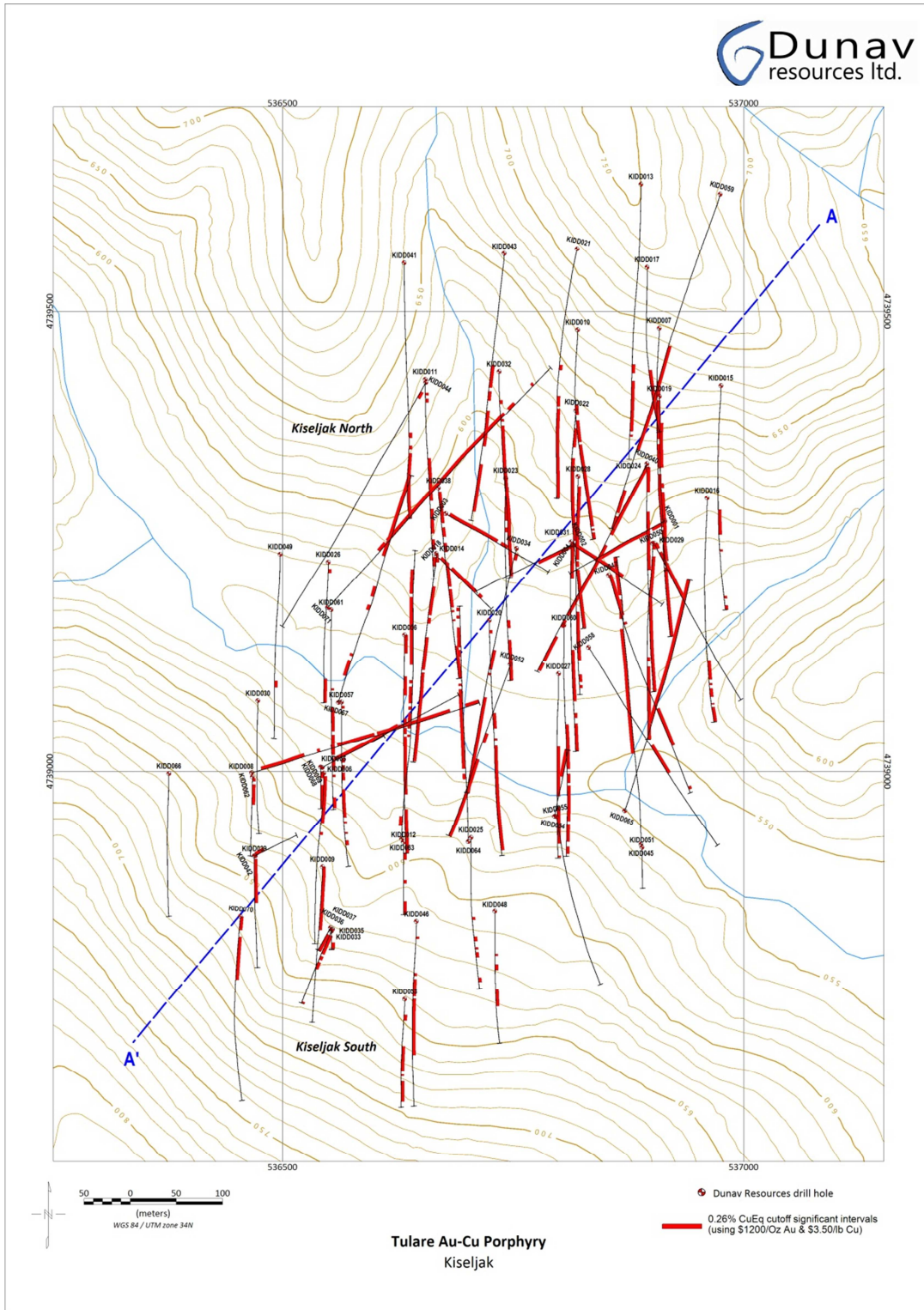
Figure 2: Plan view of the Kiseljak areas showing Dunav drilling to date (section line A-A' relates to Figure 3). Note that the grid spacing is 500 meters.
