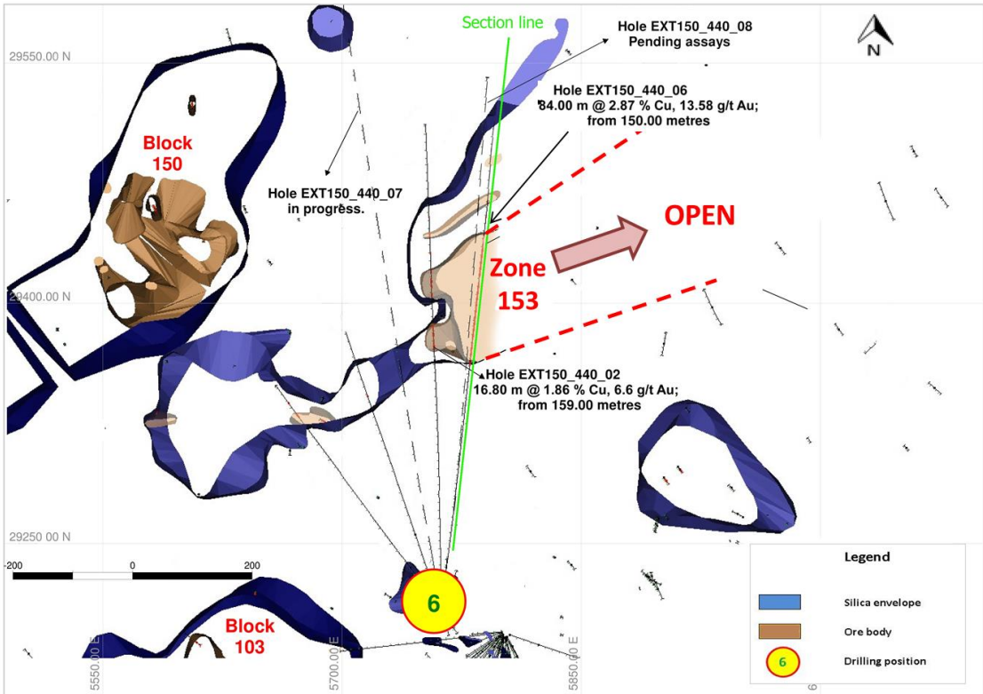
Figure 2. Plan view of current drilling position and location of Zone 153, outlined in the red box in the previous figure.
