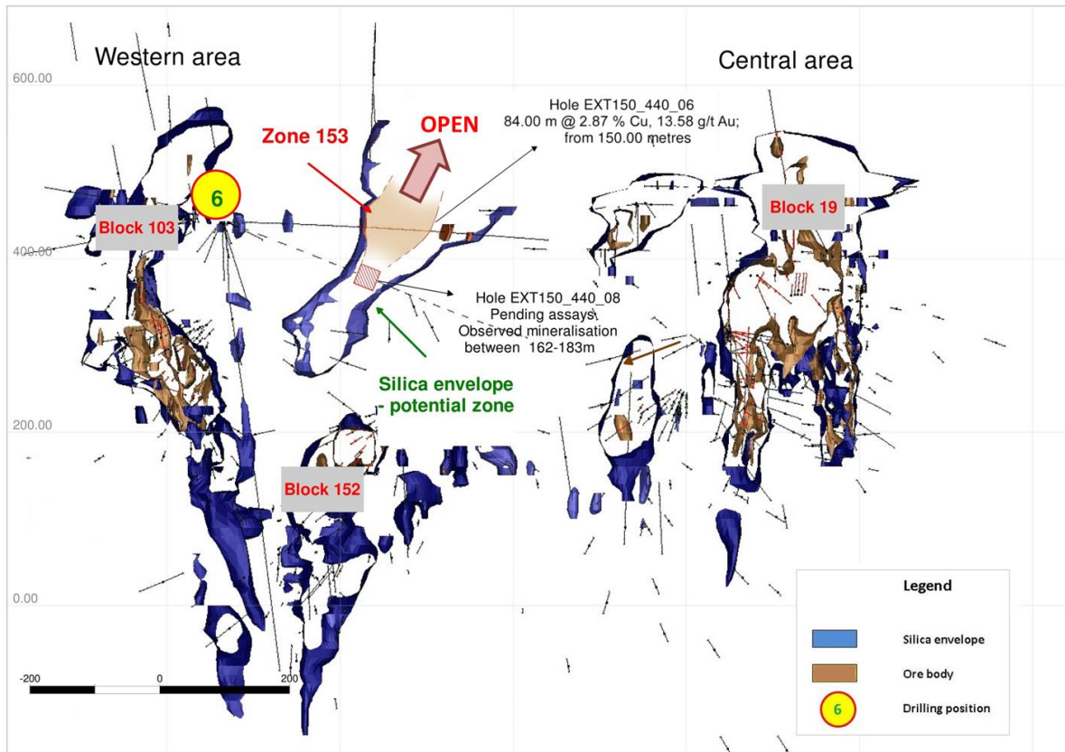
Figure 3. Cross section through the Chelopech Mine showing the location of the Zone 153 relative to the main mining blocks. The cross section is looking west. The section axis is shown on figure 2.
