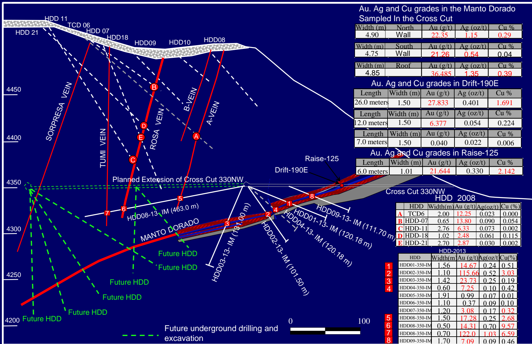
Figure 3 Tumipampa: Surface and Underground Drilling and Excavation results
