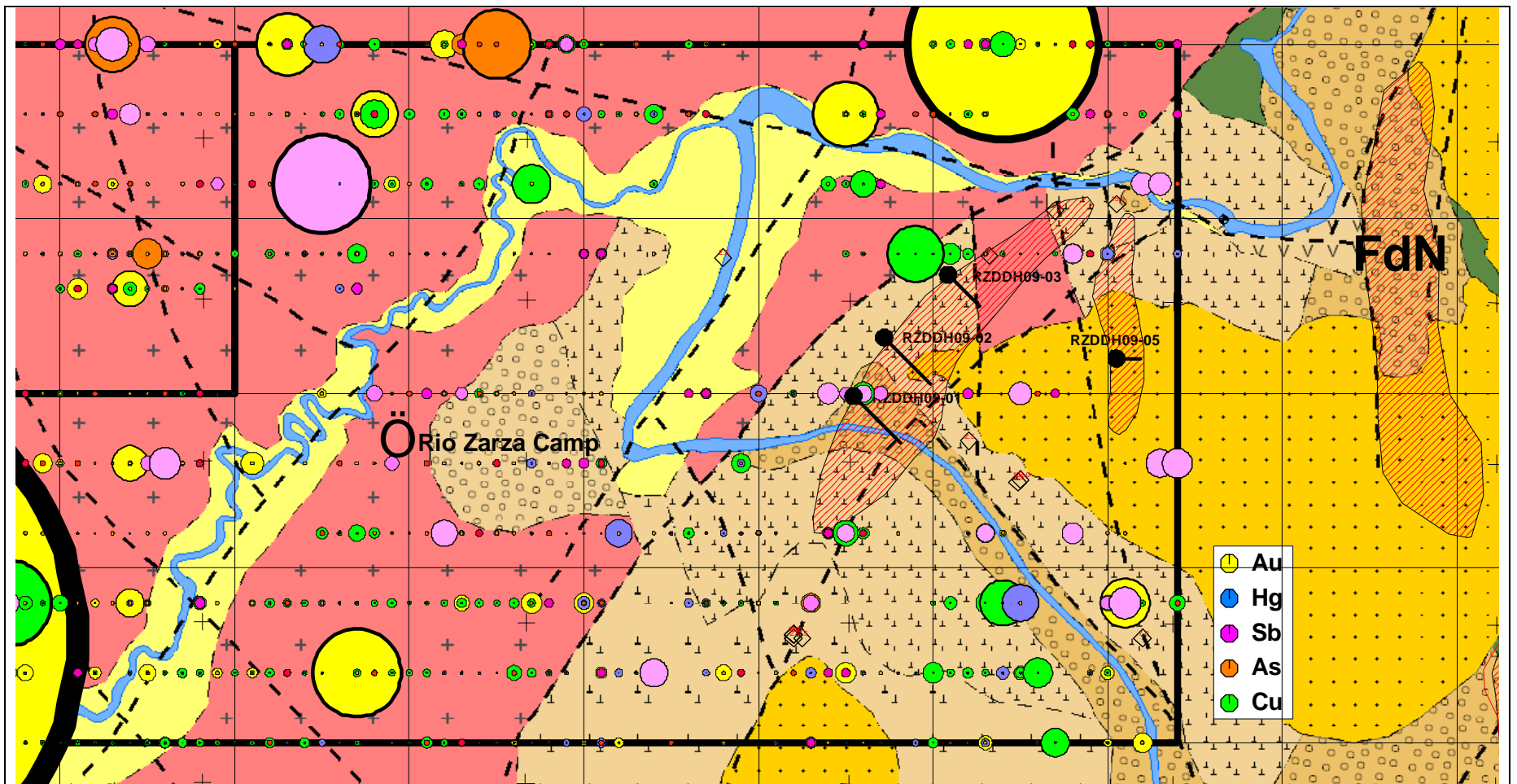
Geology map of the Rio Zarza project area showing geology, geophysical and geochemical anomalies and planned initial drill targets
