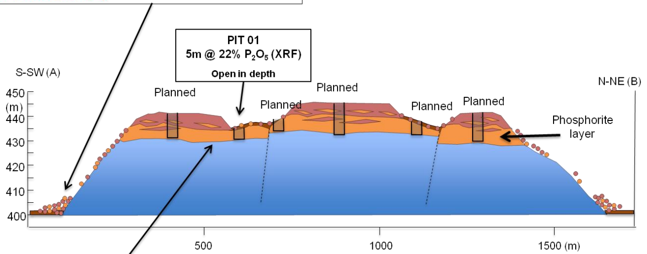
Grab and chip lab results up to 28% P 2 O 5 and the phosphorite rock types confirm XRF readings of least 5 meters at 22% P 2 O 5 in Pit 01
