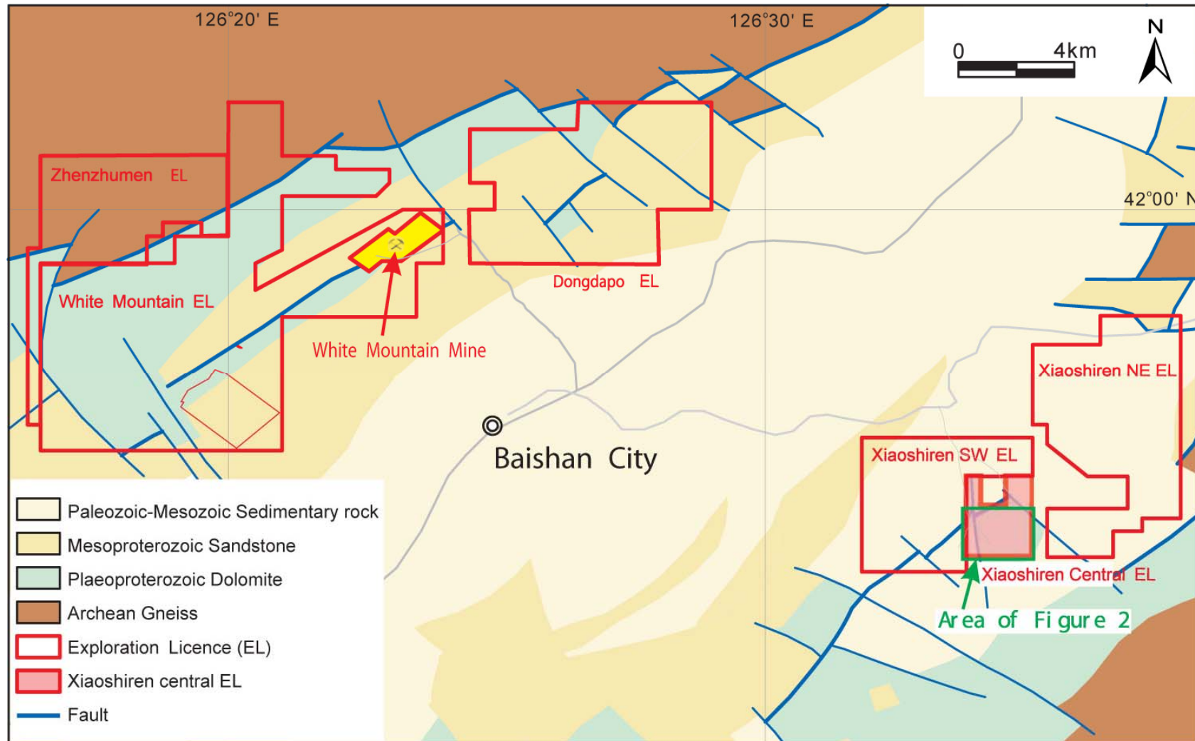
Figure 1: Locations of Xiaoshiren exploration licenses and Dongdapo exploration license relative to White Mountain Mine
