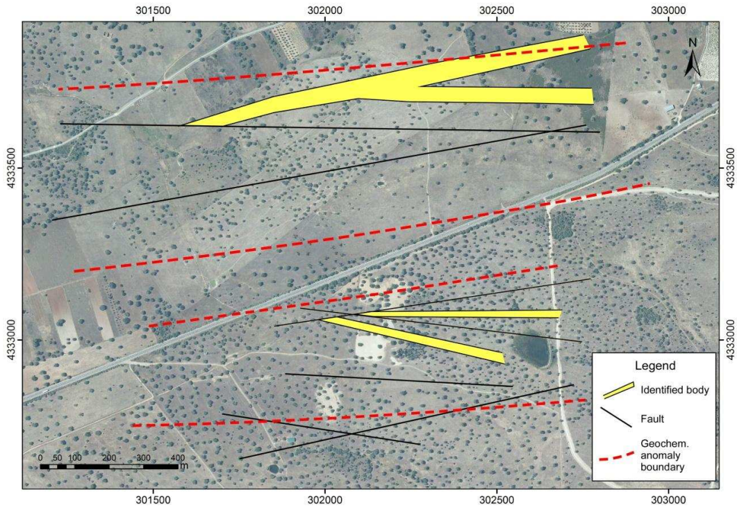
Figure 7: Identification of high resistivity and high chargeability zones and tectonic structures in the Central area of the Las Morras Property
