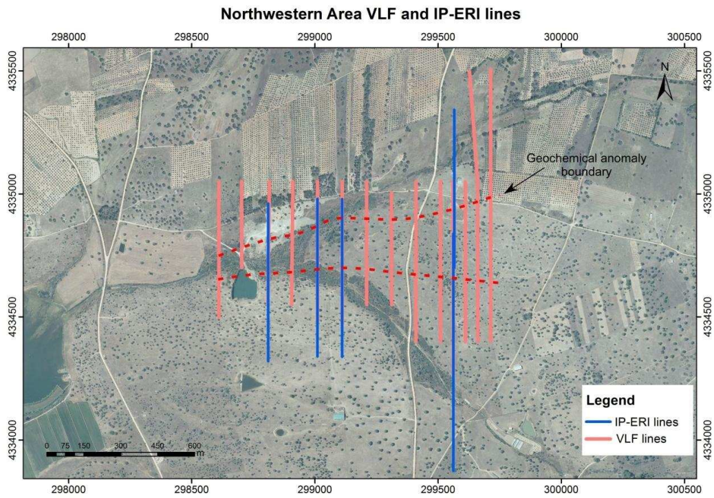
Figure 4: VLF and IP-ERT exploration lines of the Northwestern area.
