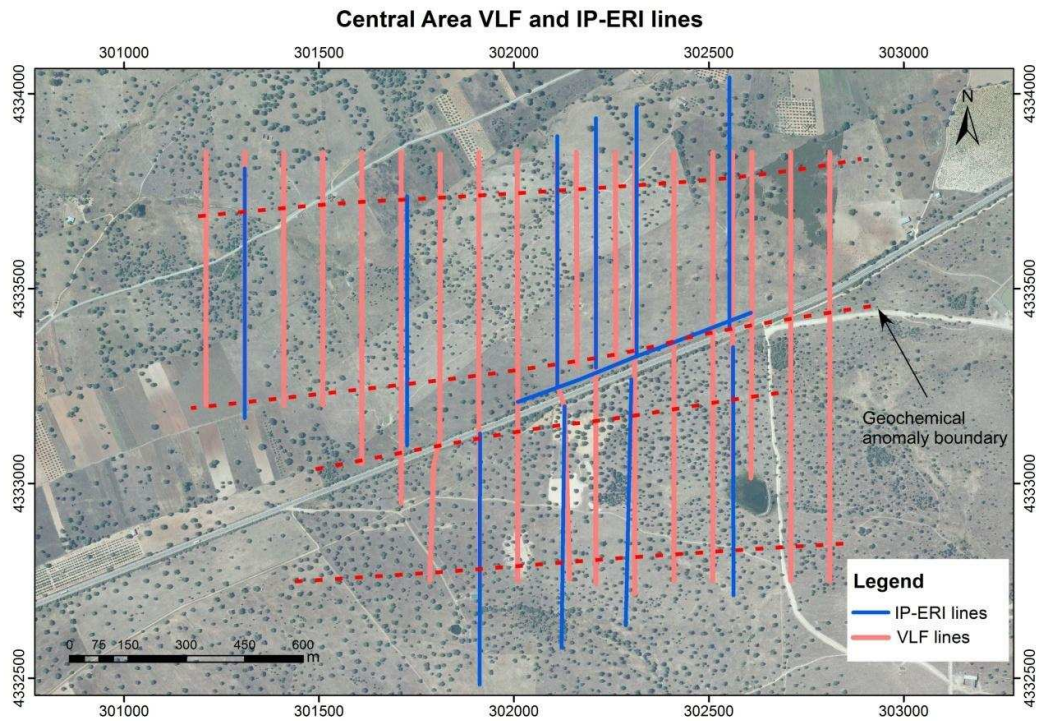
Figure 5: VLF and IP-ERT exploration lines of the Central area.
