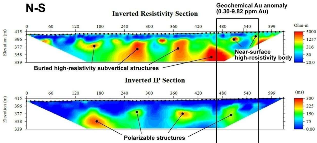
Figure 6: Example of an ERT and IP geophysical profile of the central area showing sub vertical high resistivity and high chargeability bodies.
