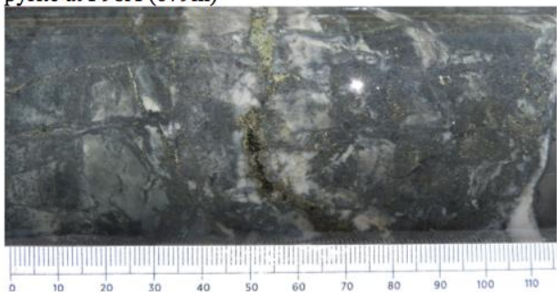
Alteration, veining, and disseminate chalcopyrite and pyrite at F98A (679m)
