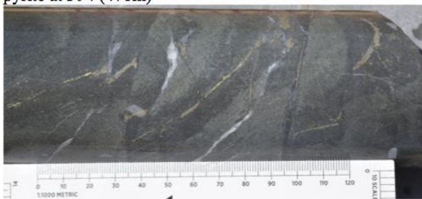
Alteration, veining, and disseminate chalcopyrite and pyrite at F98A (679m)
