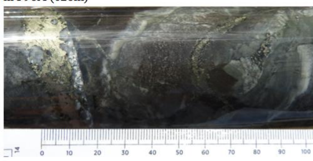
Alteration and different generation of chalcopyrite veins in F98A (628m)
