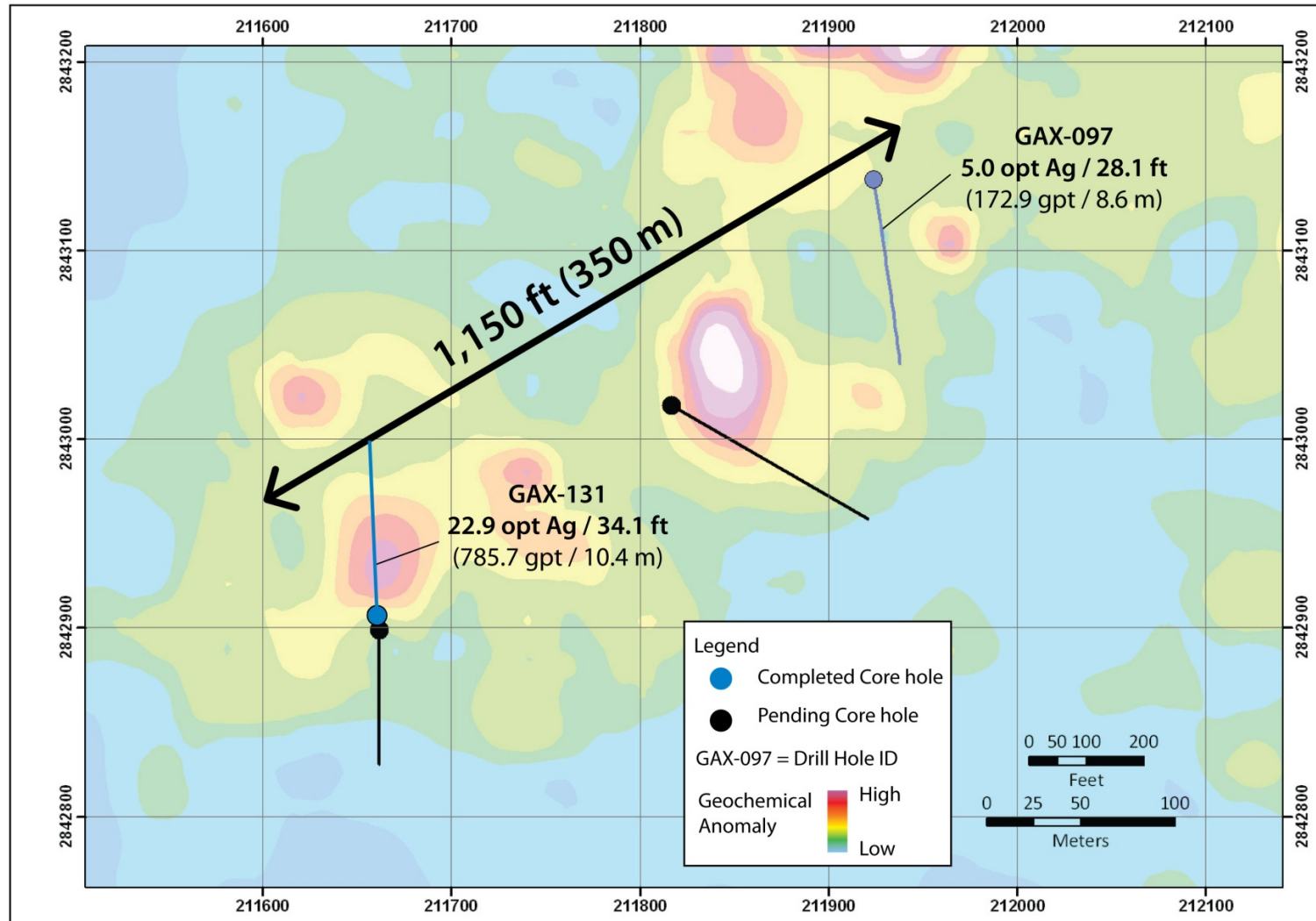
Figure 3 Southwest Zone - Current & Pending Drill Holes
