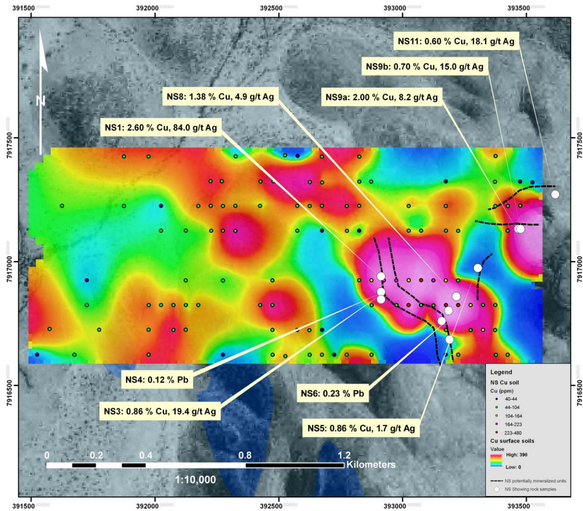
Figure 1: Contoured copper soil geochemistry (Niton readings) with rock sample localities and assays
