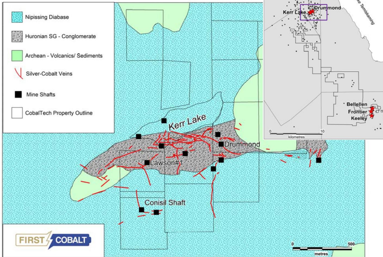
Figure 1. Bedrock geology of the Kerr Lake area. Location of silver-cobalt veins are projected to surface and based on government maps so should not be considered as exact.
