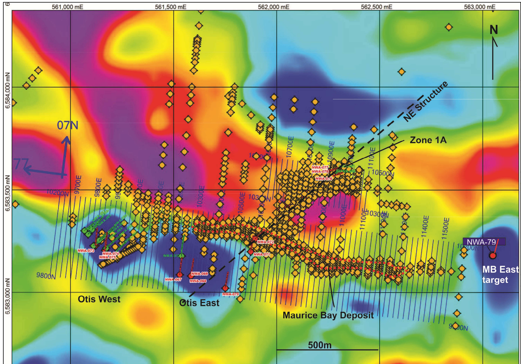
Figure 1: Map of Maurice Bay Deposit Area. The blue colours represent gravity lows, the reds are gravity highs. Yellow dots are historical holes, most of which were stopped at the unconformity. Green dots are 2012/13 drill holes. The red dots are the drill holes completed in 2014.
