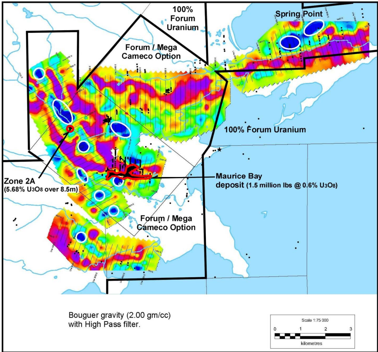
Figure 1: Filtered Bouguer Gravity on the NW Athabasca Project. Gravity lows are in dark blue, drill target areas are circled. The black dots show the location of existing drill holes. Most of the gravity lows have not been drill tested. The light blue colour is Lake Athabasca.
