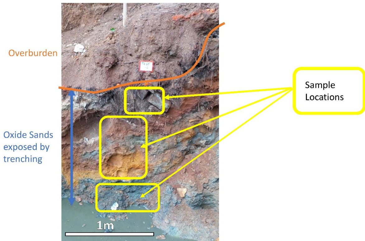
Figure 1 - Systematic sampling of the units composing the soil formation to characterize the precious metal distribution
