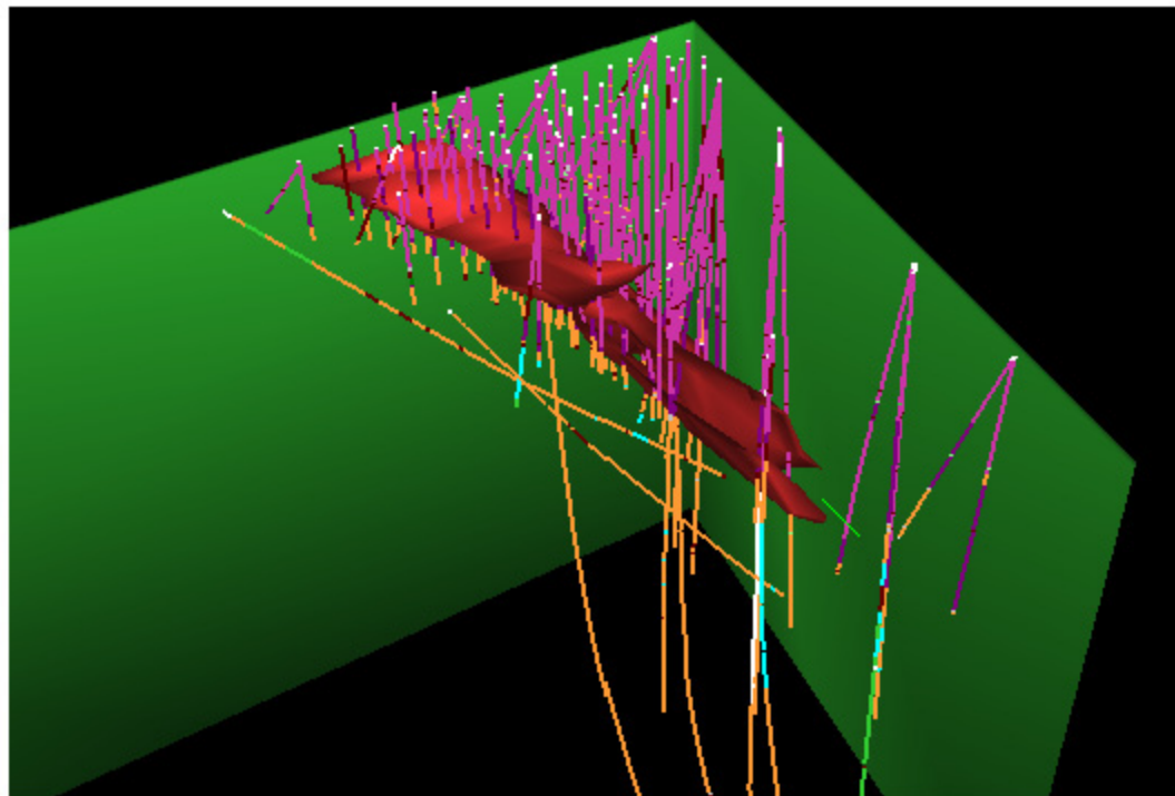
3D SCREEN CAPTURE OF THE MINERALIZED WIREFRAME OF THE CONWEST ZONE View is to the northwest. The property boundary is in green.
