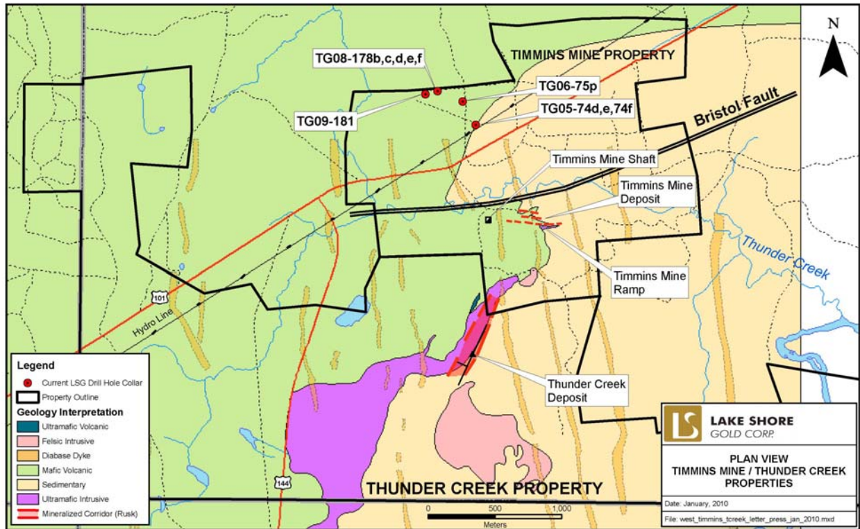
Figure 3. Plan View
