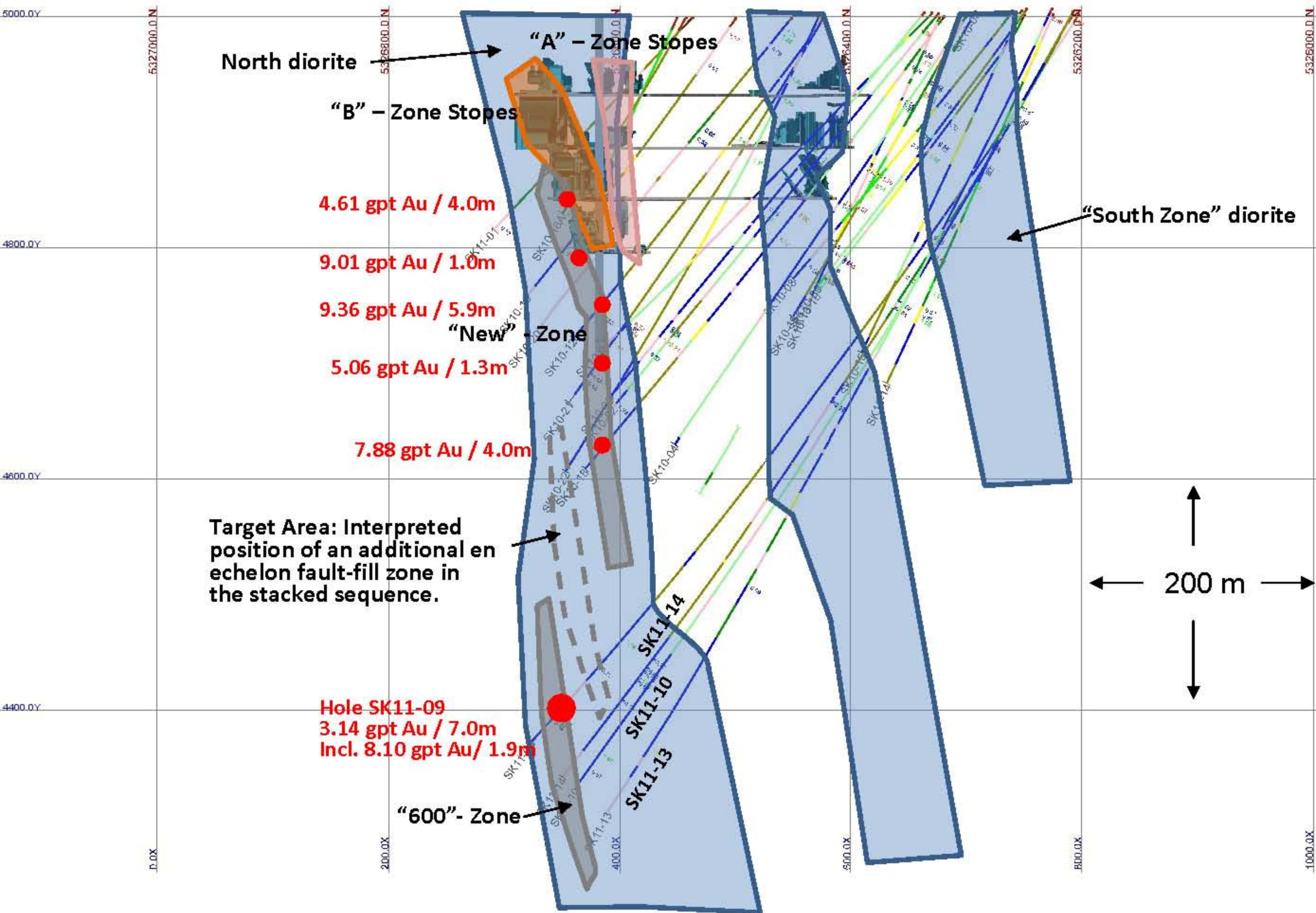
Figure 1: Composite Cross Section (Facing East) – Simkar Project Projected drill holes are from 2010 and 2011 exploration campaigns only
