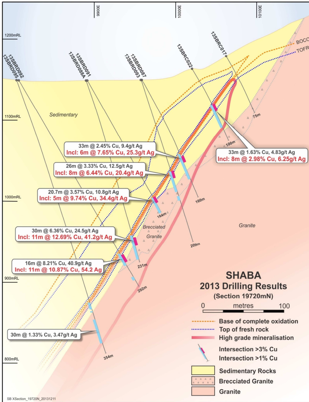
Figure 2: Drill cross-section through Shaba deposit
