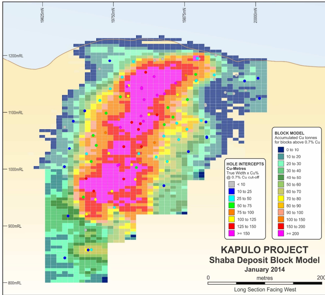
Figure 3: Shaba deposit long-section looking west, shown as a 2-dimensional representation of the resource block model with blocks coloured by accumulated copper tonnes in blocks grading 0.7% Cu or greater.
