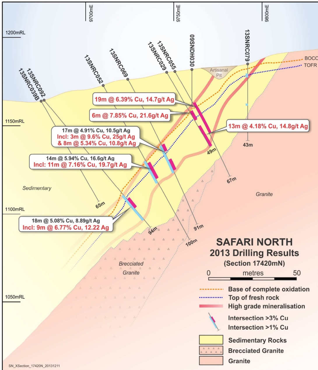
Figure 4: Drill cross-section through Safari North deposit
