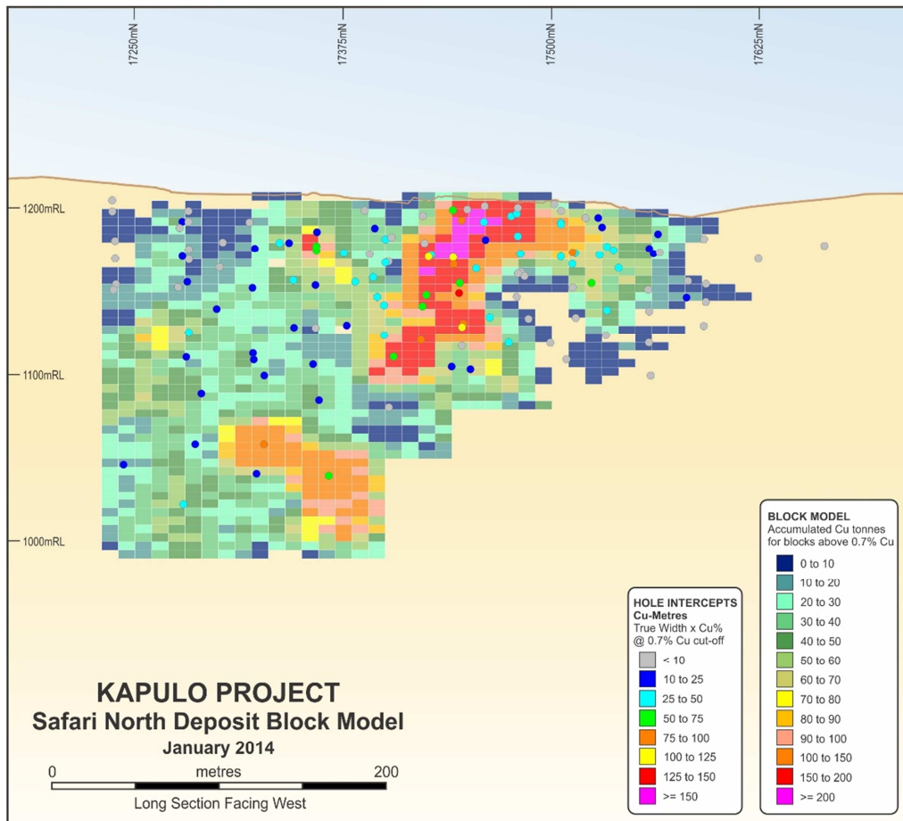
Figure 5: Safari North deposit long-section looking west, shown as a 2-dimensional representation of the resource block model with blocks coloured by accumulated copper tonnes in blocks grading 0.7% Cu or greater.
