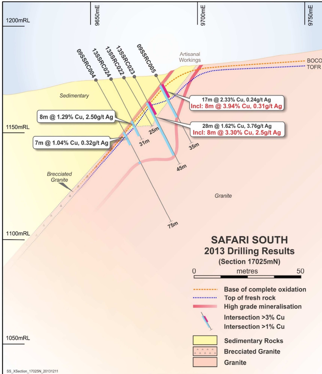
Figure 6: Drill cross-section through Safari South deposit
