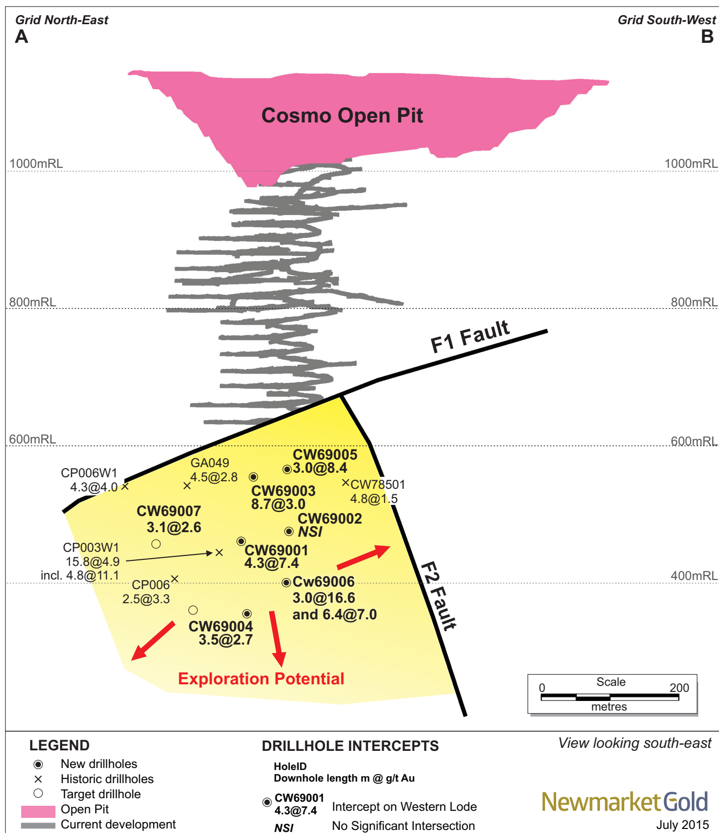
Figure 2 Longitudinal Projection of Cosmo Western Lodes, Cosmo Gold Mine
