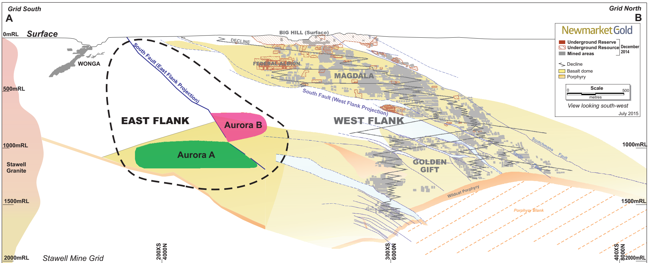
Figure 5 Longitudinal Projection of Stawell Gold Mine showing East Flank Targets
