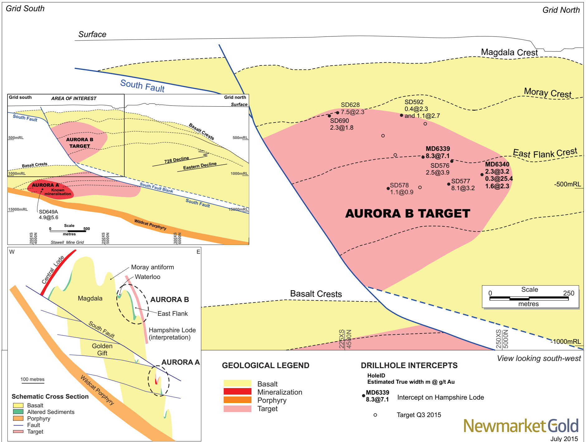
Figure 6 Longitudinal Projection of East Flank Targets, Stawell Gold Mine
