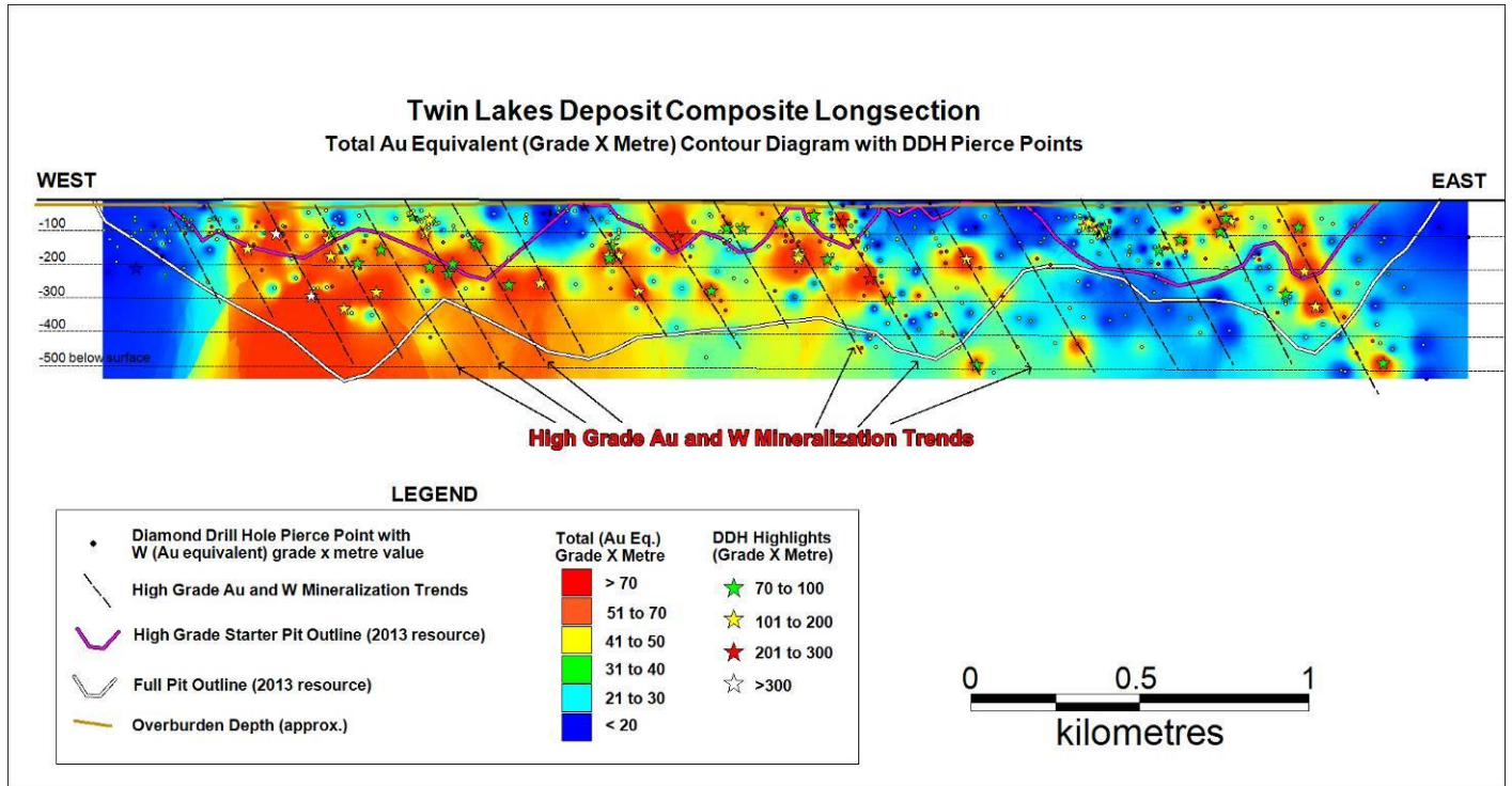
Figure 1: Twin Lakes Deposit Composite Long Section – Total Au Equivalent (Grade X Metre) Contour Diagram with DDH Pierce Points – Showing Consistent High Grade Gold and Tungsten Cores Combined
