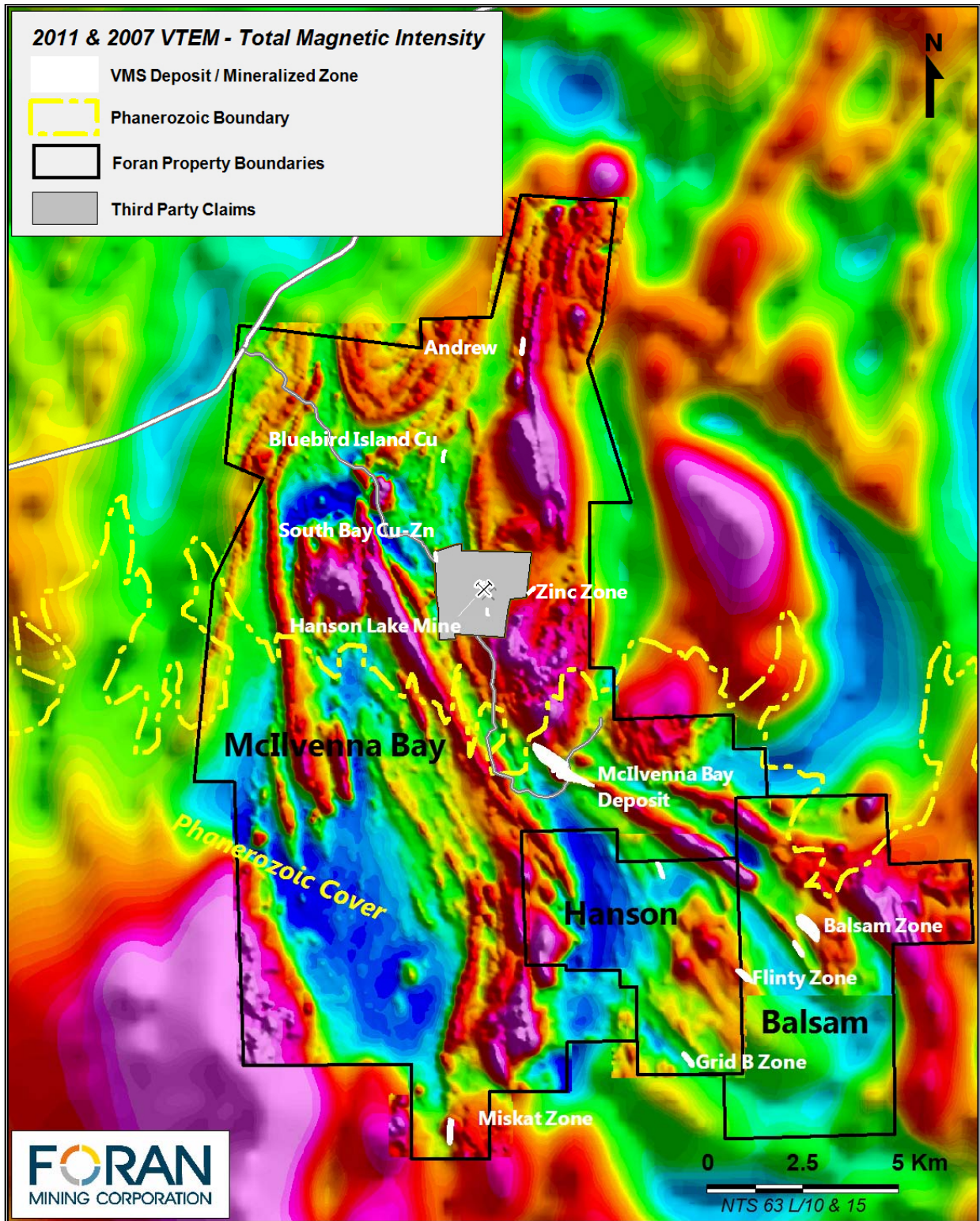
Figure 1. Total Magnetic Intensity (TMI) of 2011 and 2007 VTEM surveys for Foran's McIlvenna Bay, Balsam and Hanson properties.
