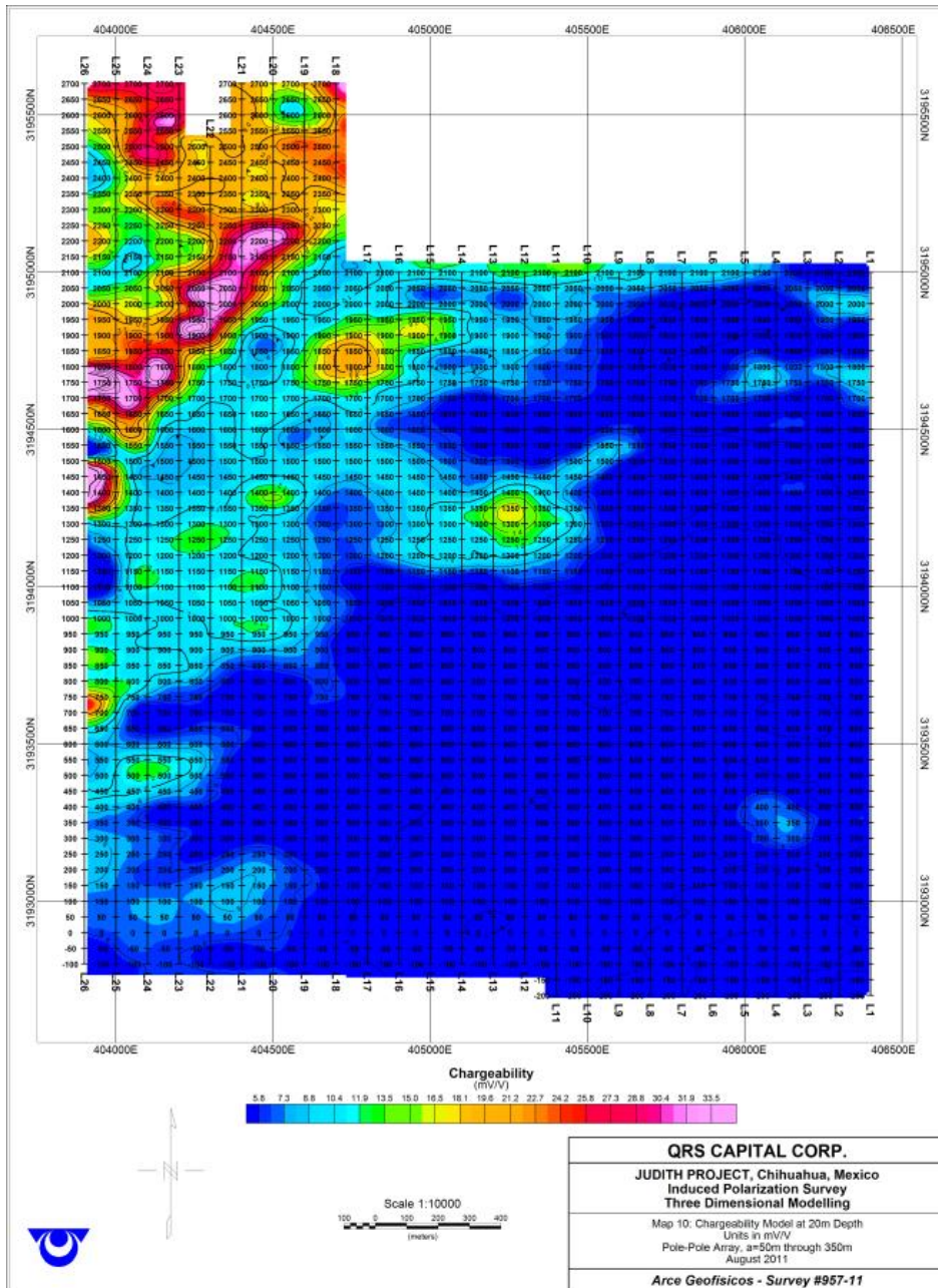
Figure 10 - Chargeability anomalies are evident on the Northwest portion of the survey area, corresponding to the low SP response and the various low resistivity masses in that section of the survey area
