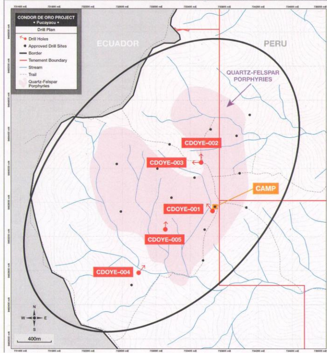
Figure 2: Drill Locations
