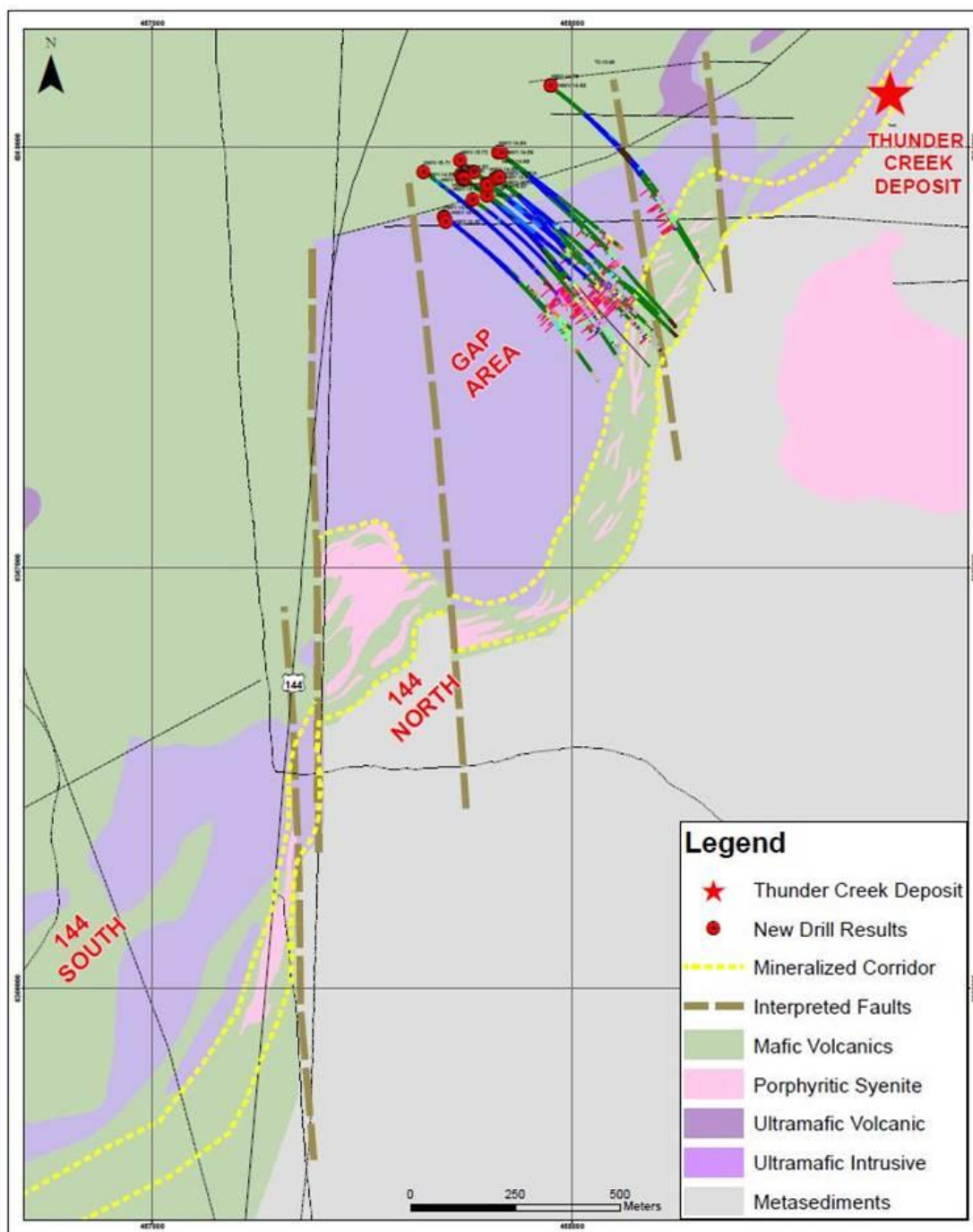
Figure 1. 144 Geology Plan – Location of New Drill Holes
