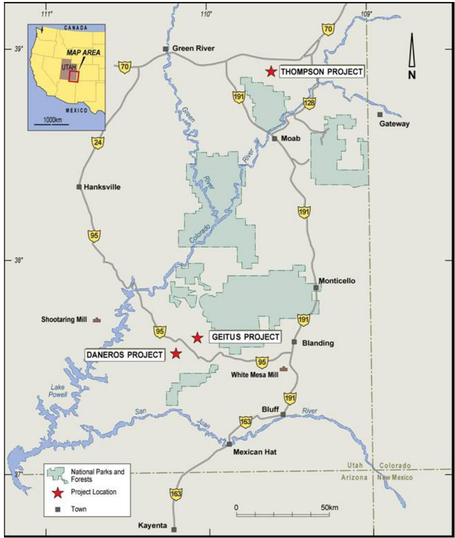
Figure 1: Location of Daneros Deposit.
