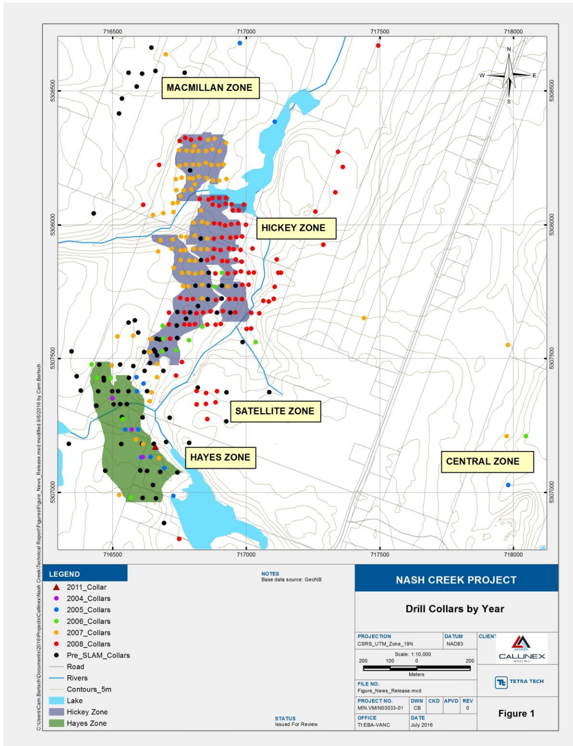
Figure 1: Nash Creek Plan Map with Drill Collars
