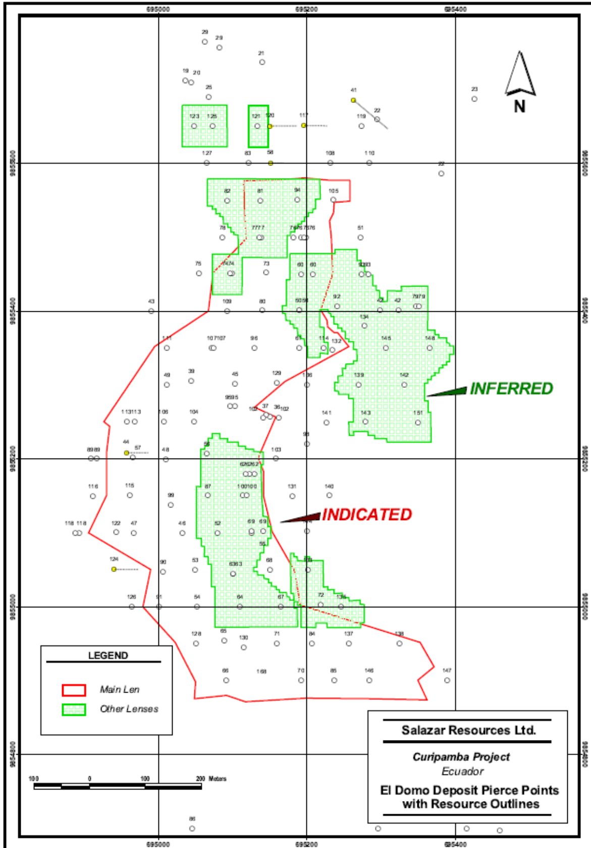
Figure 1: El Domo Pierce Points Map with Resource Outlines
