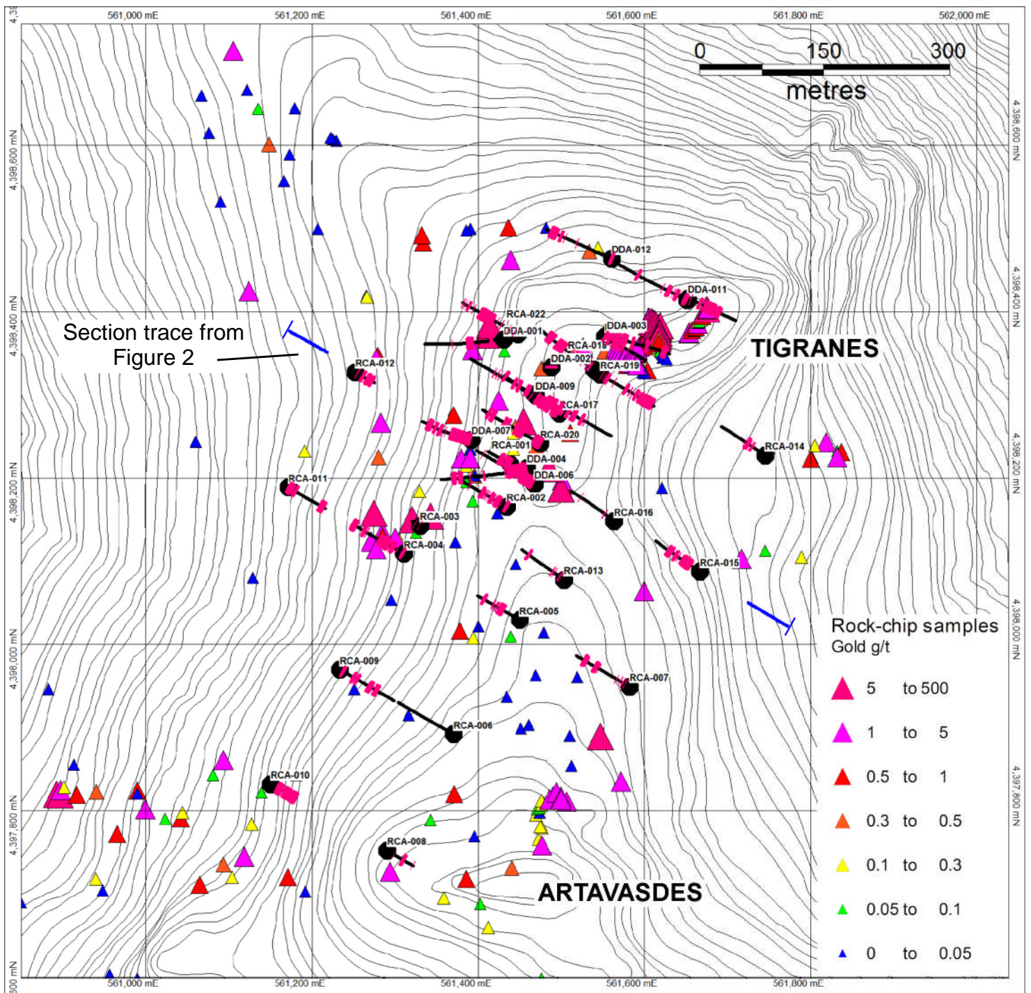
Figure 1. Plan projection of drill holes and surface rock-chip geochemistry from the Tigranes and Artavasdes areas; Amulsar Project, Armenia. Drill intersections projected to the surface (indicated by purple bars) show intersections greater than 0.5g/t.
