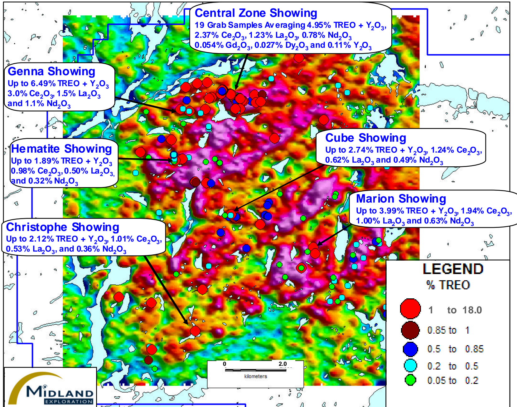
Figure 2. Ytterby 3 Grab Sample Results on Thorium Radiometric Map
